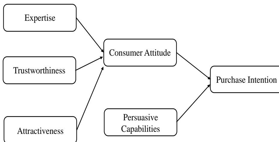
Figure 2.1. Theoretical Framework
